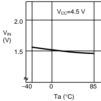
1.8 Input voltage V_{IN} – Ambient temperature T_a S-24H Series : All inputs S-24S Series : CE, SK and DI
